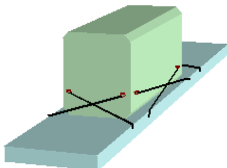
Figure 7.38 Direct lashing against sliding
